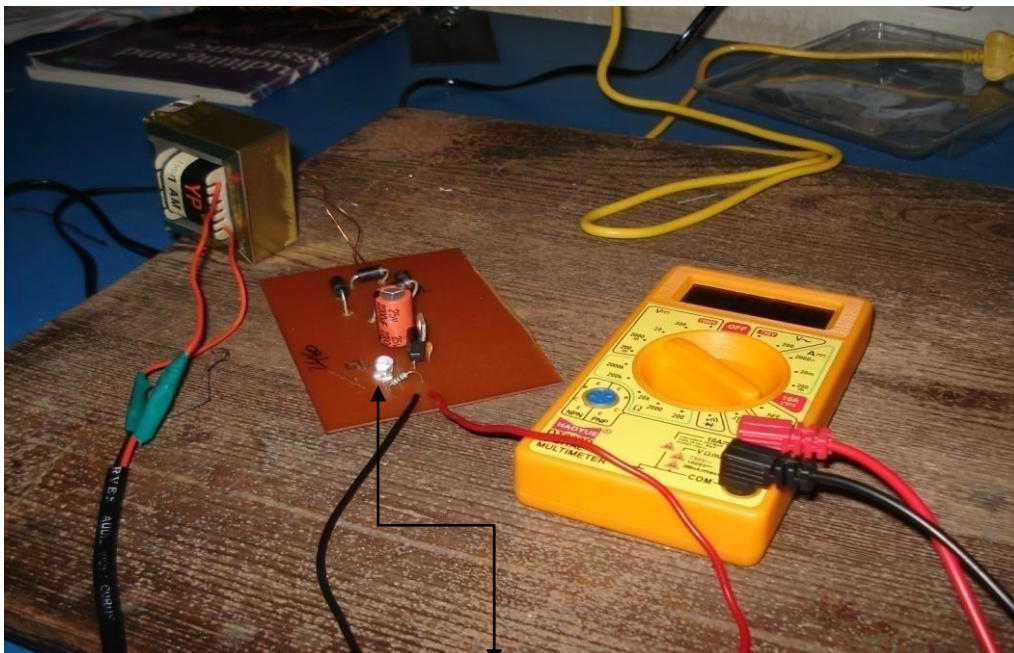
5 V Regulated Power Supply Circuit testing by glowing LED
